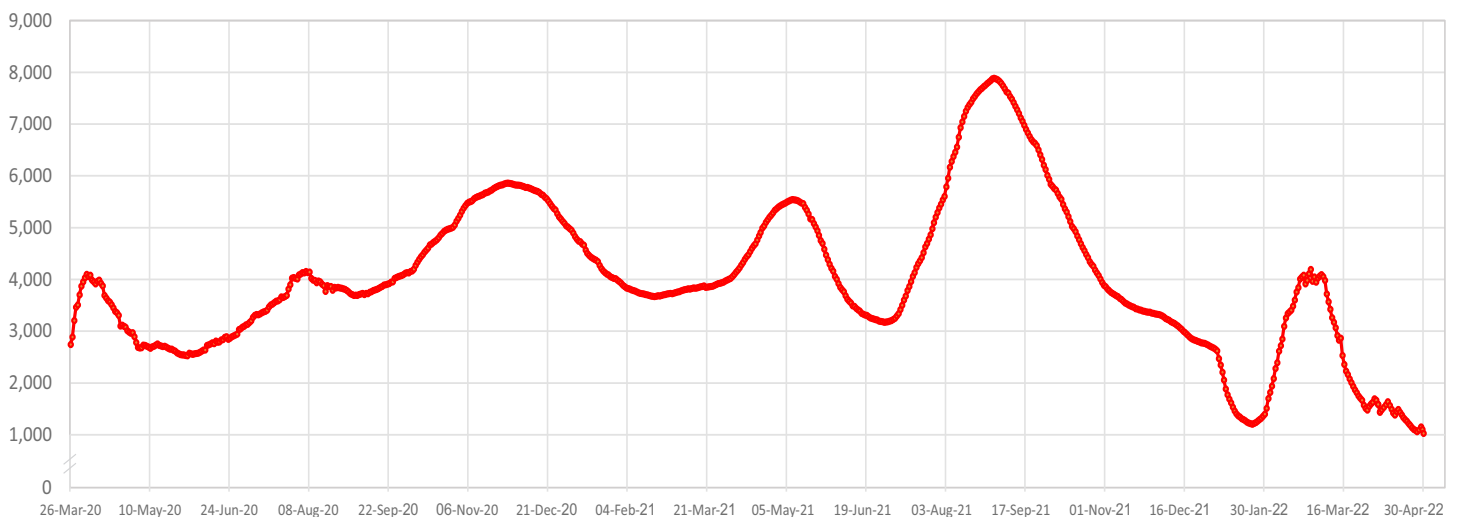
Figure 2 - COVID-19 Patients in Intensive Care, 26 March 2020 - 01 May 2022
