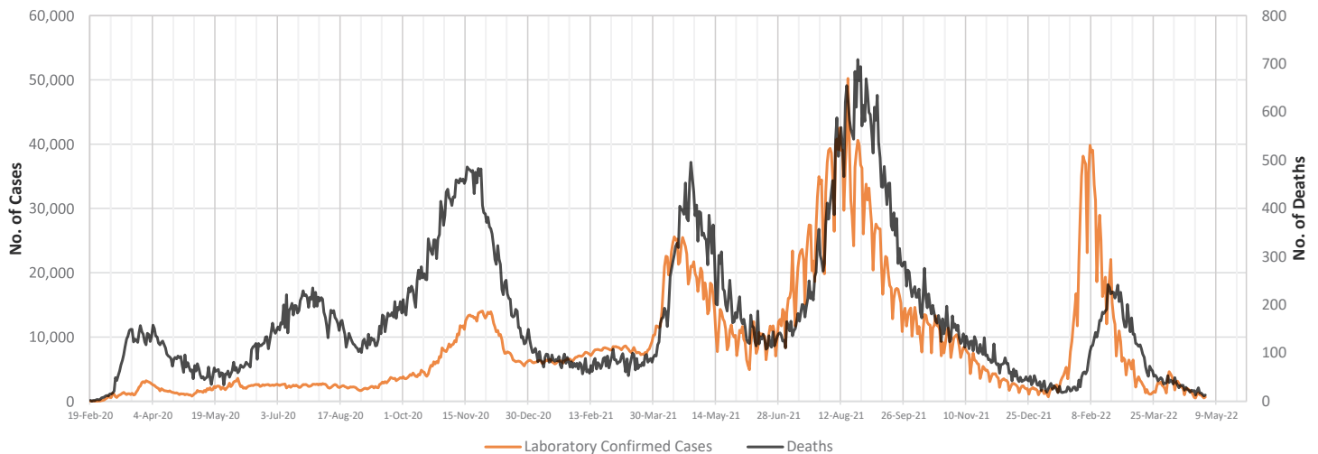
Figure 1 - Trend of COVID-19 Laboratory-Confirmed Cases and Deaths, 19 February 2020 - 01 May 2022
