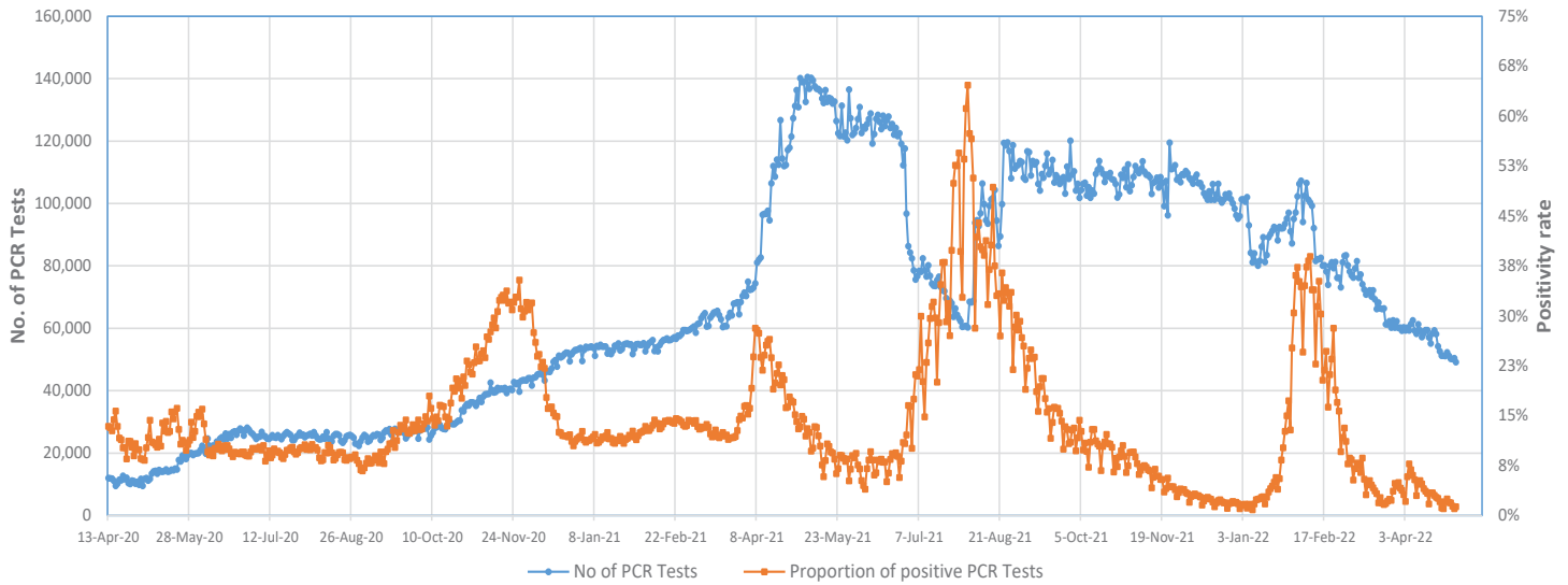
Figure 3 - Number of Daily COVID-19 PCR Tests and Percentage of Positive Cases, 13 April 2020 - 01 May 2022
