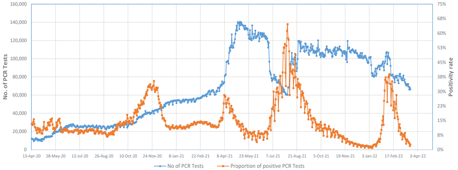
Figure 3 - Number of Daily COVID-19 PCR Tests and Percentage of Positive Cases, 13 April 2020 - 20 March 2022
