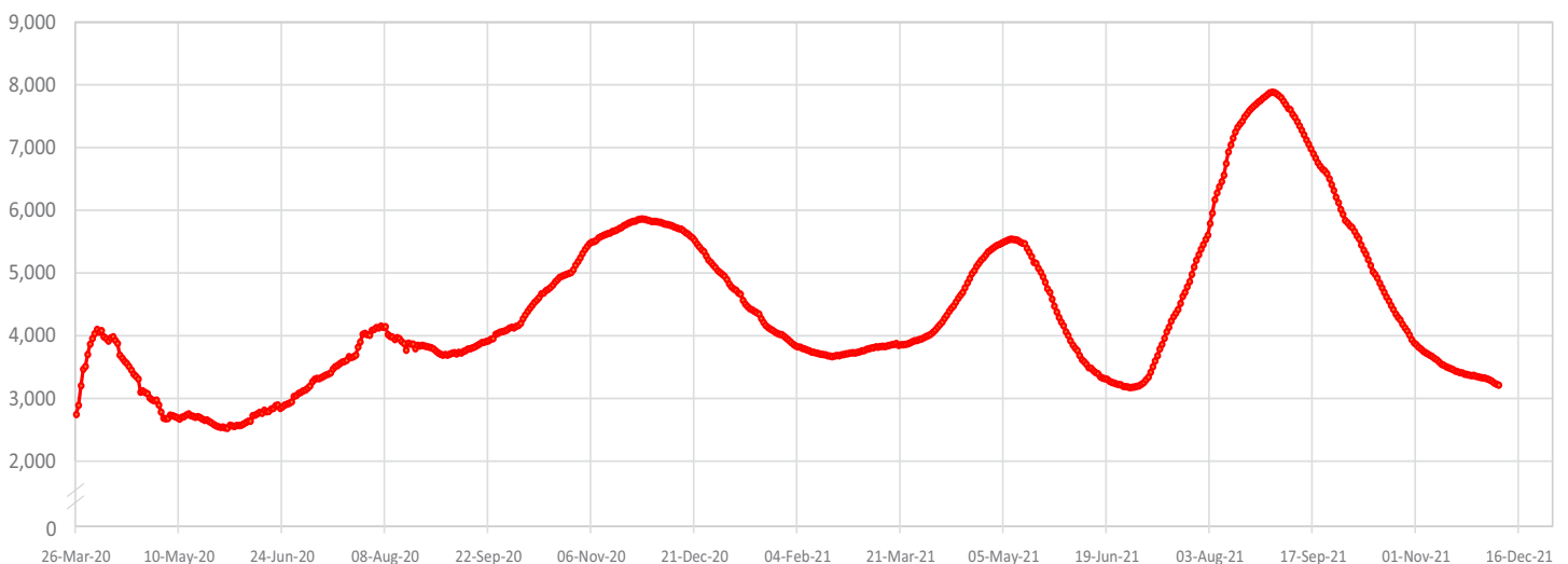
Figure 2 - COVID-19 Patients in Intensive Care, 26 March 2020 - 07 December 2021
