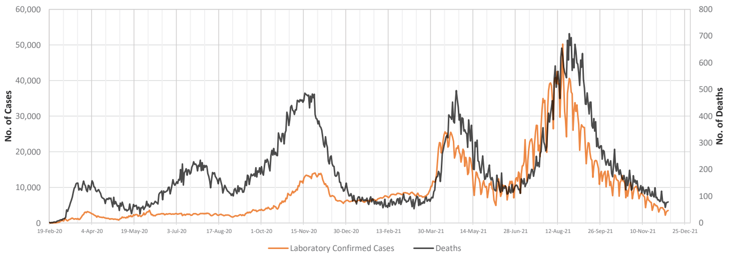
Figure 1 - Trend of COVID-19 Laboratory-Confirmed Cases and Deaths, 19 February 2020 - 07 December 2021
