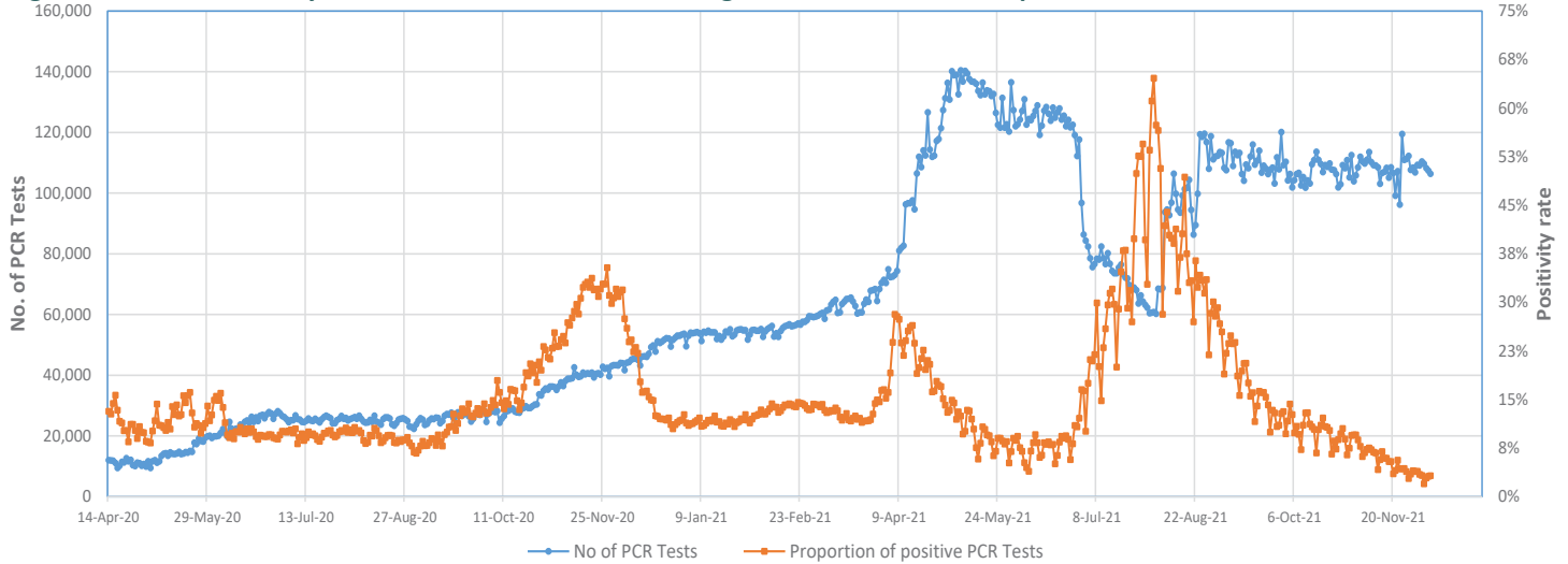
Figure 3 - Number of Daily COVID-19 PCR Tests and Percentage of Positive Cases, 13 April 2020 - 07 December 2021
