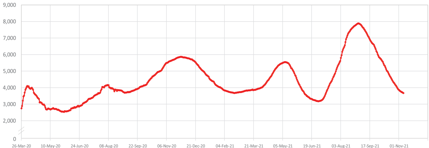
Figure 2 - COVID-19 Patients in Intensive Care, 26 March 2020 - 08 November 2021
