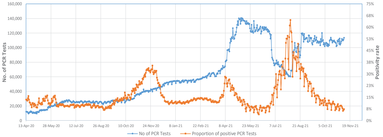
Figure 3 - Number of Daily COVID-19 PCR Tests and Percentage of Positive Cases, 13 April 2020 - 08 November 2021
