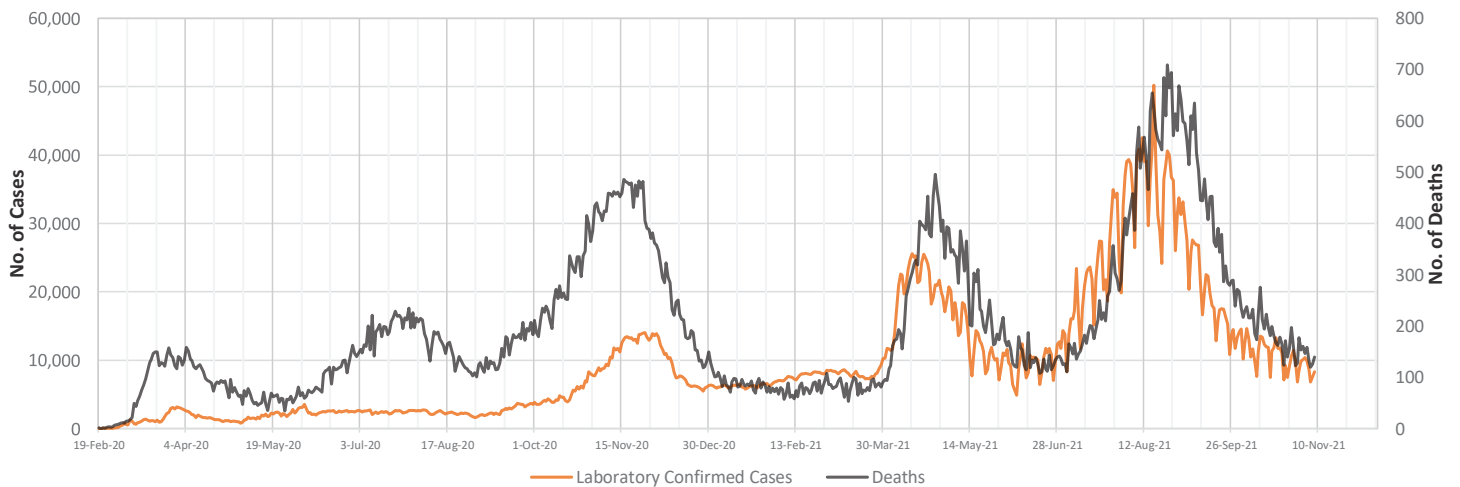
Figure 1 - Trend of COVID-19 Laboratory-Confirmed Cases and Deaths, 19 February 2020 - 08 November 2021
