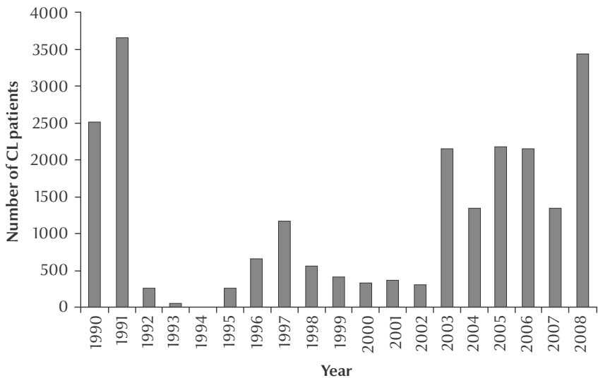
Figure 1 Annual incidence of cutaneous leishmaniasis due to Leishmania major in
