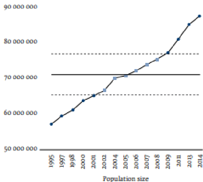
Figure 1 Control charts of number of dental graduates, population size and dentist availability, 1995- 2014
