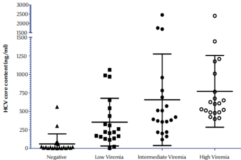
Figure 1 Scattergram of HCV core antigen values with the mean and standard deviation among the 4 viraemia groups (based on HCV RNA levels as described in the text). The difference between the groups was statistically significant ( P < 0.001 )
