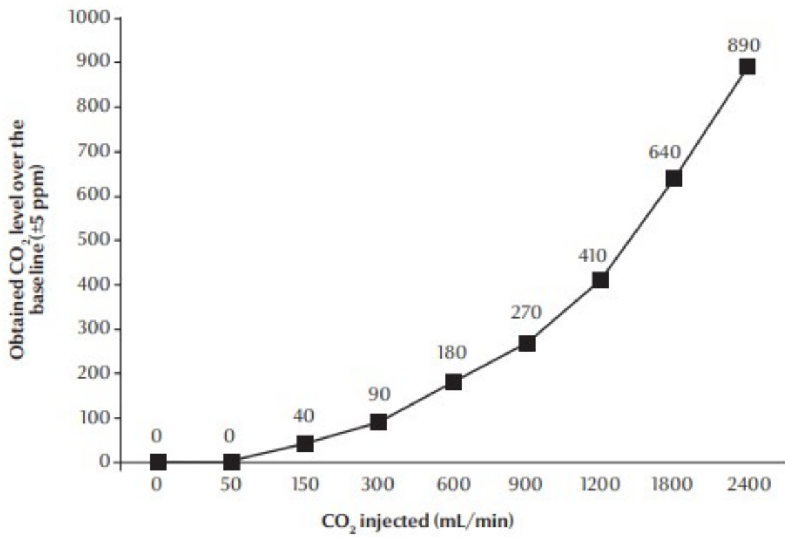
Figure 1 Flow concentration function for CO 2 2% injection in the wind tunnel over the background level
