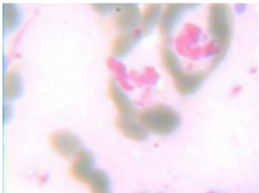
Figure 4 Microscope image shows amastigotes released into extracellular fluid with elevation in the number of neutrophils and phagocytosis activity
