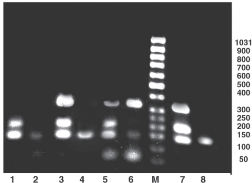
Figure 1 Agarose gel electrophoresis of multiplex polymerase chain reaction products of Bacillus anthracis isolates (Bac = B. anthracis chromosome; PA = protective antigen; Cap = capsule)
