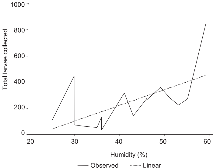
Figure 3 Relationship between immature stages of Anopheles arabiensis and relative humidity, March 1999–June 2000
