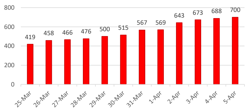
Total Number of Cases
