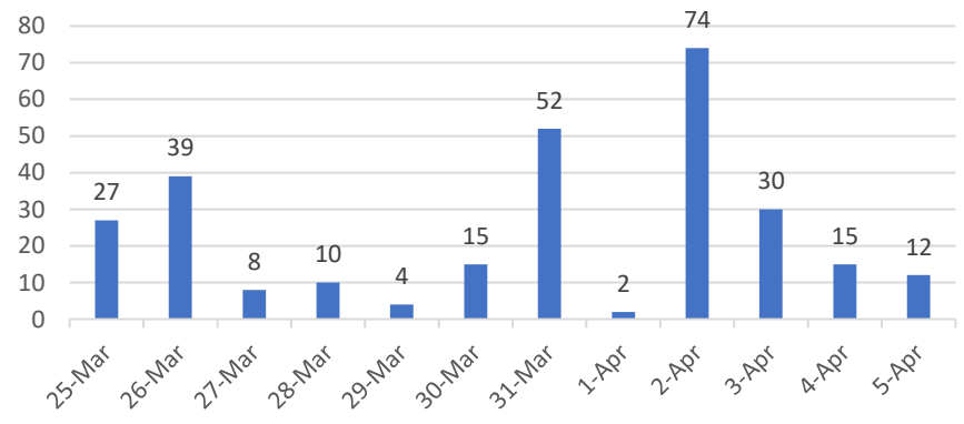
Number of New Cases
